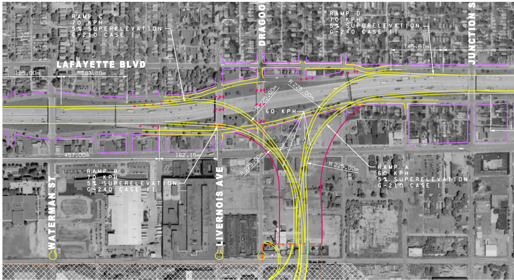
VP Interchange 3 Exhibit 7.6
